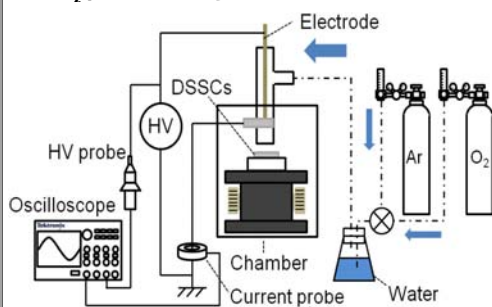
Fig. 1 An experimental setup for TiO 2 sample surface modification.
