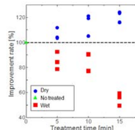
Fig. 5 Effect of humidity in the carrier gas.
