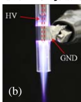
Fig. 2 (b) image of Ar + O 2 plasma discharge.
