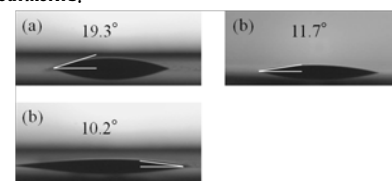
Figure 6. The appearance of water droplet on TiO 2 surface. (a) Untreated (b) Dry treated (c) Wet treated
