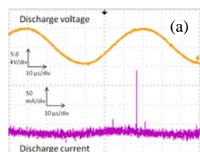
Fig. 2 (a) current-voltage wave form.
